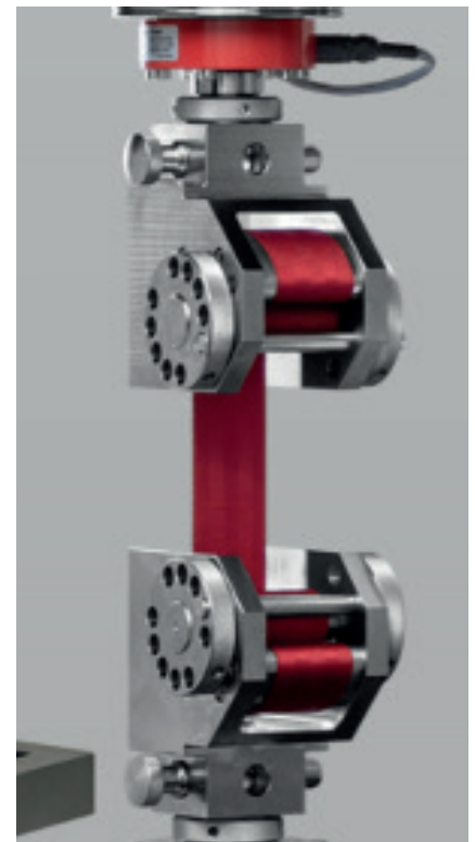
Fig. 2. Tensile test on belts
