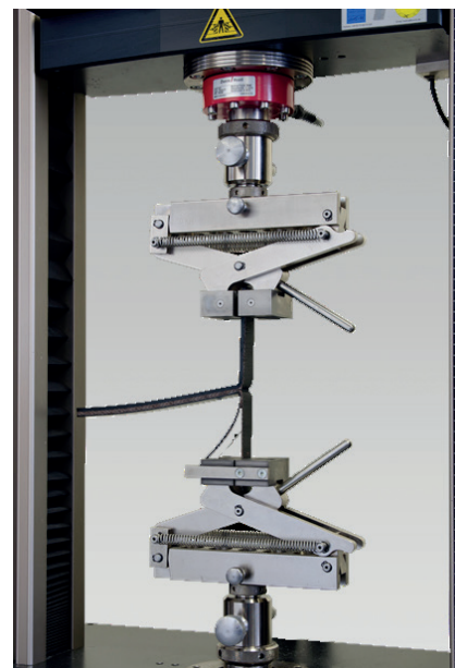
Fig. 2. Adhesion test to determine the adhesive strength between constitutive elements
