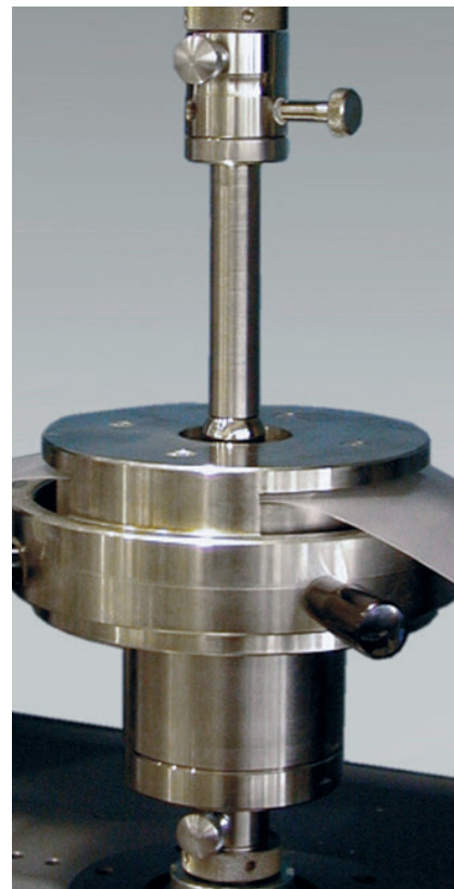
Fig. 3. Bursting strength
